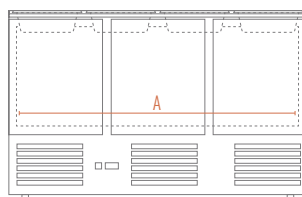
SALADETTE SF 901 BC FRONTE / FRONT
